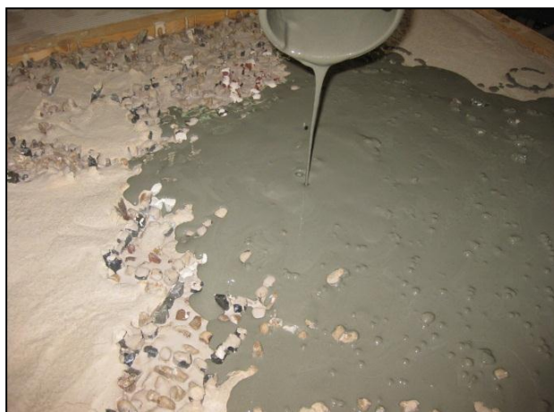
11 a, b. The aspect of the surface after the first layer of fine roman cement was casted
