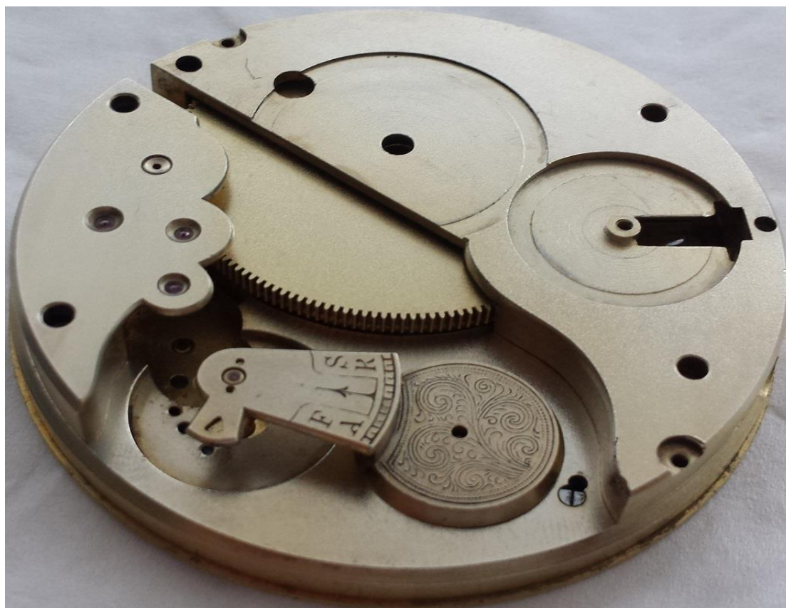
16. movement parts assembled after cleaning
