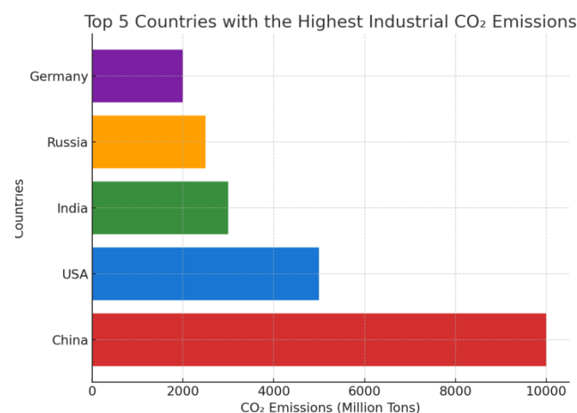
Fig.4: Top 5 countries with the highest industrial CO 2 emissions
