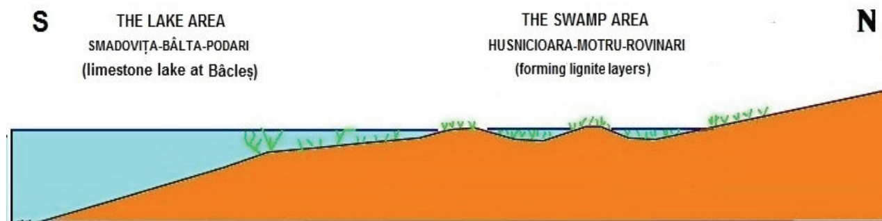
Figure 3. S – N section through the region west of the Jiu River during the Pelendavian stage.
