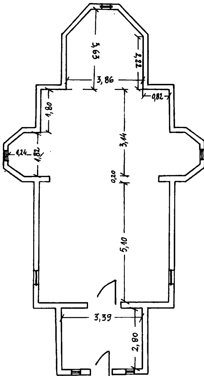
Plan 1/100
