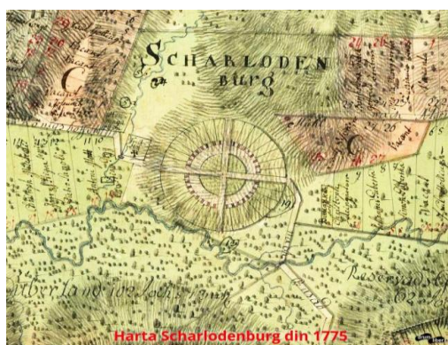
Fig.1. Charlottenburg map
