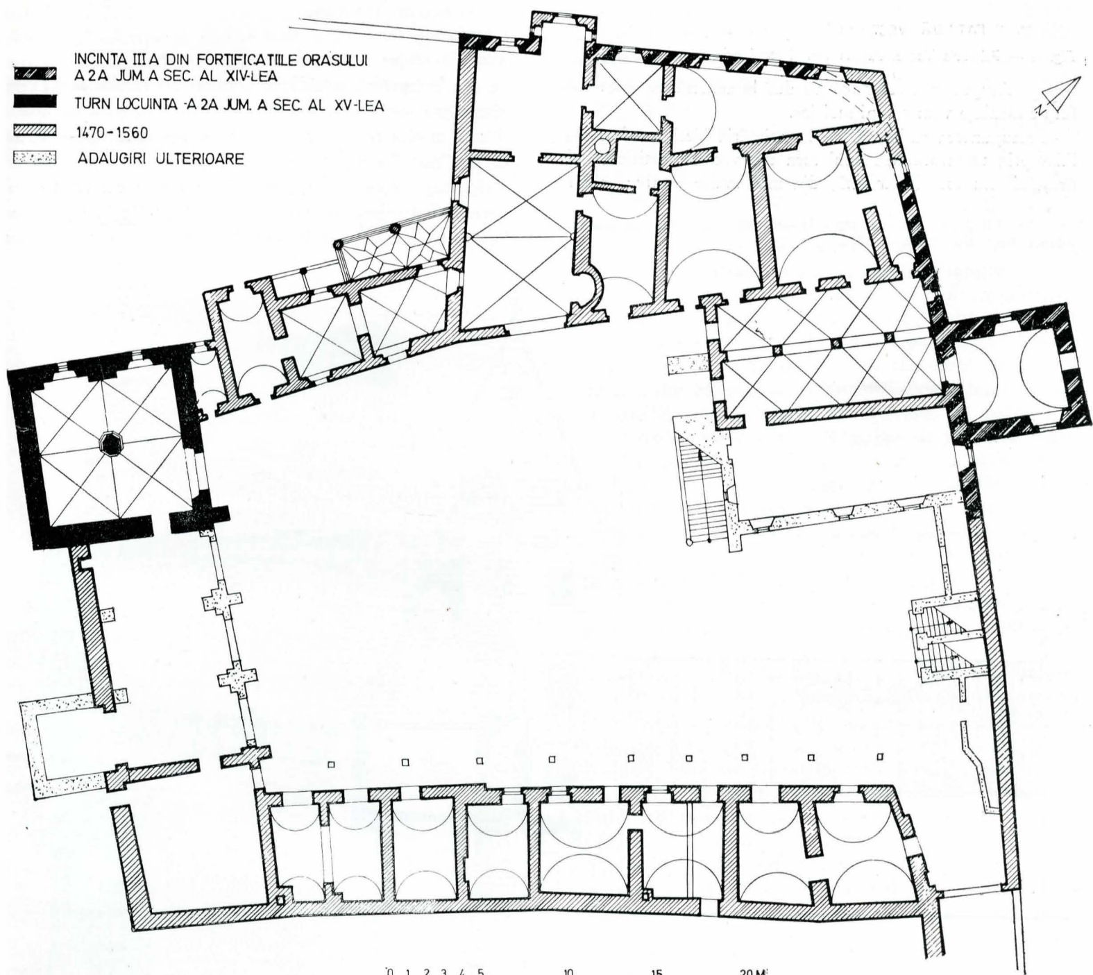
PLAN PARTER
