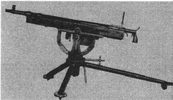
Fig. 15 Mitraliere Colt - Browning, model 1895/1914, calibrul 7,62 mm
